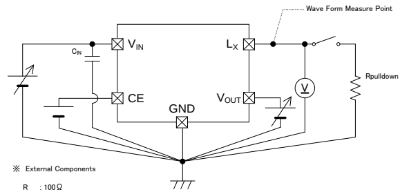
< Test Circuit No.2 >
