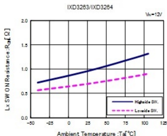
(8) Lx SW ON Resistance vs. Ambient Temperature
