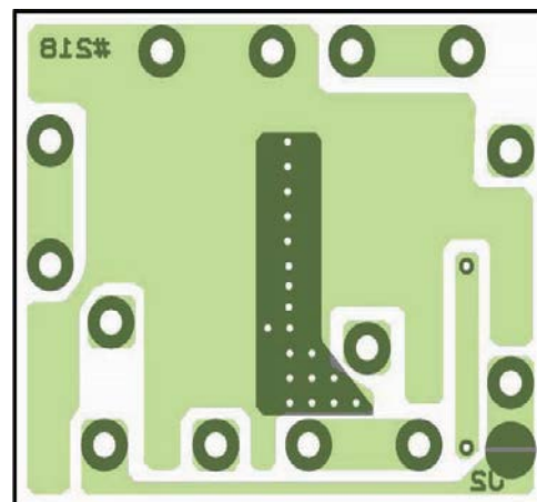
USP-6C (Back)
