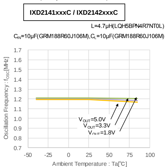
(16) Oscillation Frequency vs. Ambient temperature
