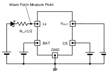
< Circuit No.⑥ >
