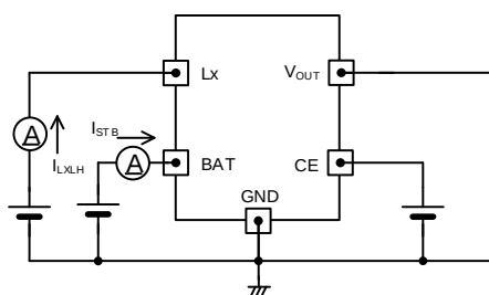
< Circuit No.⑧ >
