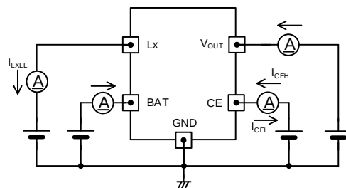
< Circuit No.② >
