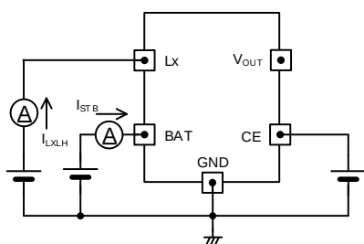
< Circuit No.⑦ >
