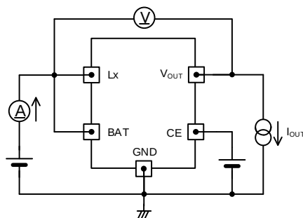
< Circuit No.④ >
