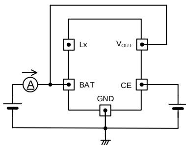
< Circuit No.③ >
