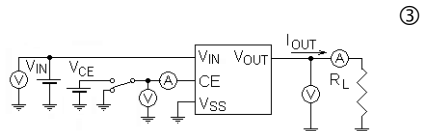
Circuit
