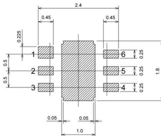
USP-6B Reference Pattern Layout, Units: mm
