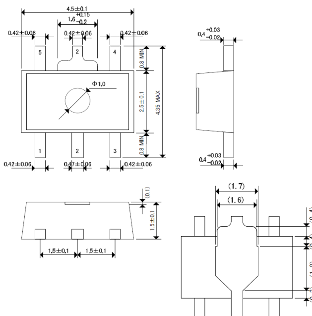
SOT-89-5, Units: mm
