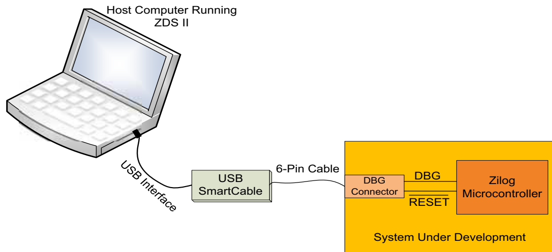
Figure 97. Development System
