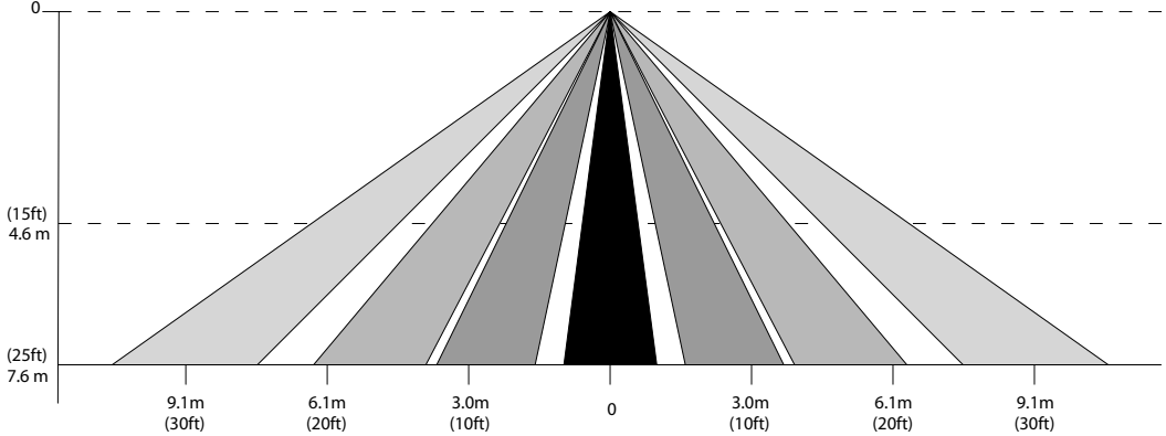
Figure 11. The ZCWM05GIV1 Lens Specification: Ceiling Mount, #2 of 2
