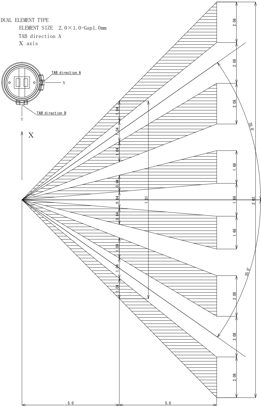
Figure 24. The ZNCL10IL Lens Specification, Tab Direction A, X Axis
