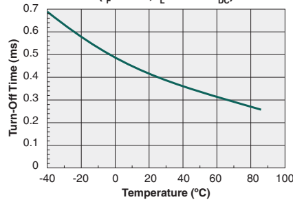
Typical Turn-Off Time vs. Temperature ( I_F=5mA, I_L=200mA_{DC} )
