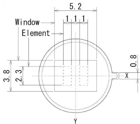
Figure 6 - Top View
