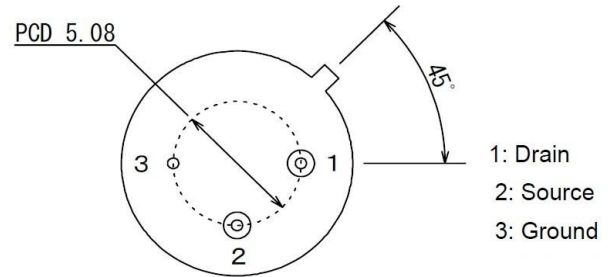
Figure 7 - Bottom View
