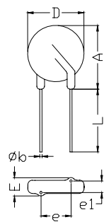
Straight Lead
