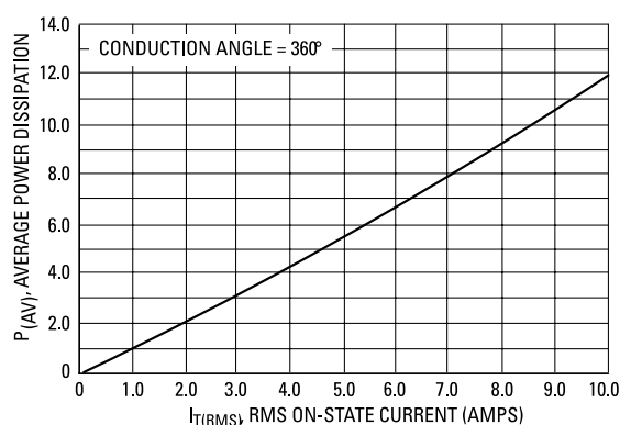
Figure 2. Power Dissipation
