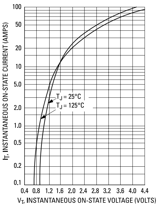
Figure 3. Maximum On-State Characteristics
