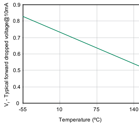
Figure 5 - Forward Voltage
