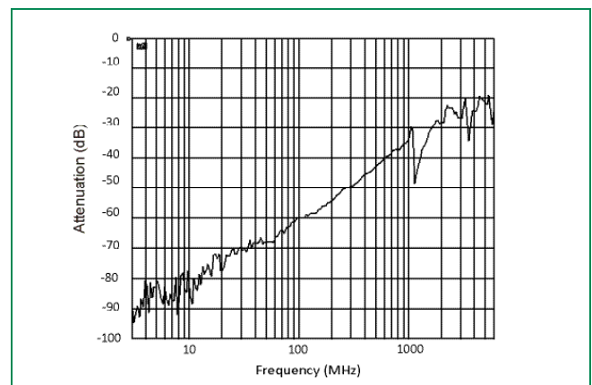
Analog Crosstalk (S41)
