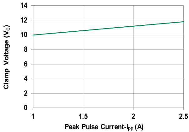
Clamping Voltage vs. IPP for 8/20µs Waveshape
