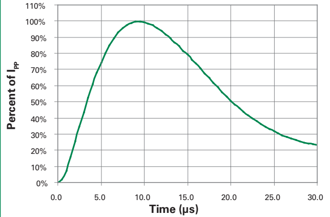
8/20 µs Pulse Waveform
