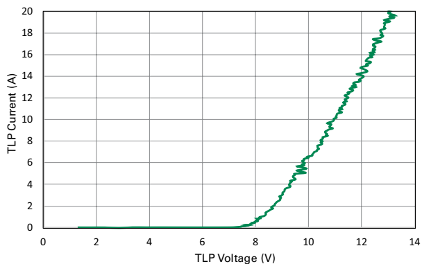
Transmission Line Pulsing(TLP) Plot
