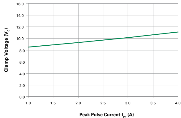
Clamping Voltage vs. I_{pp}
