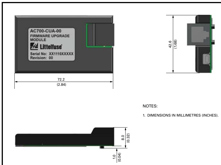
FIGURE 1. Firmware Upgrade Module (AC700-CUA-00) Outline.
