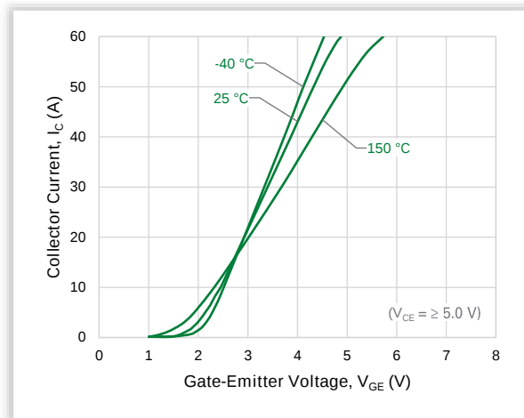
Figure 8. Transfer Characteristics
