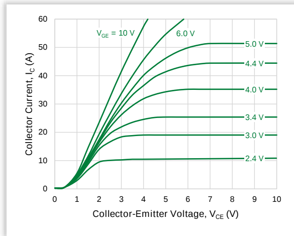
Figure 7. Output Characteristics ( T_J = 150^\circ\text{C} )
