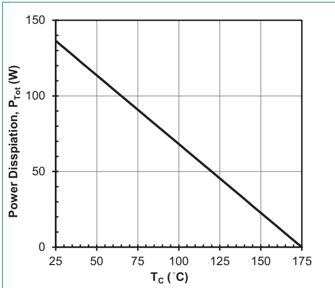
Figure 3: Power Disipation
