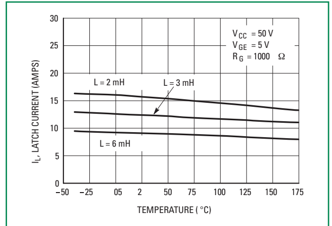
Figure 10. Minimal Open Secondary Latch Current vs Temperature
