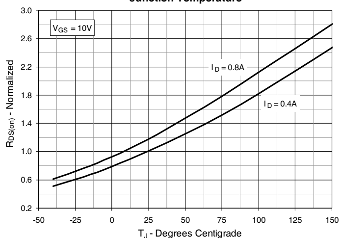
Fig. 4. R_{DS(on)} Normalized to I_D = 0.4\text{A} Value vs. Junction Temperature
