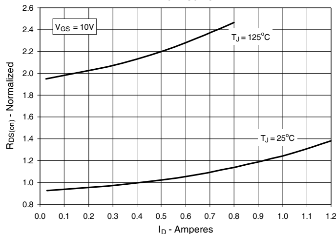
Fig. 5. R_{DS(on)} Normalized to I_D = 0.4\text{A} Value vs. Drain Current
