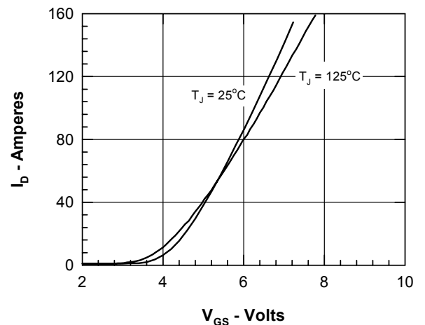
Figure 6. Admittance Curves
