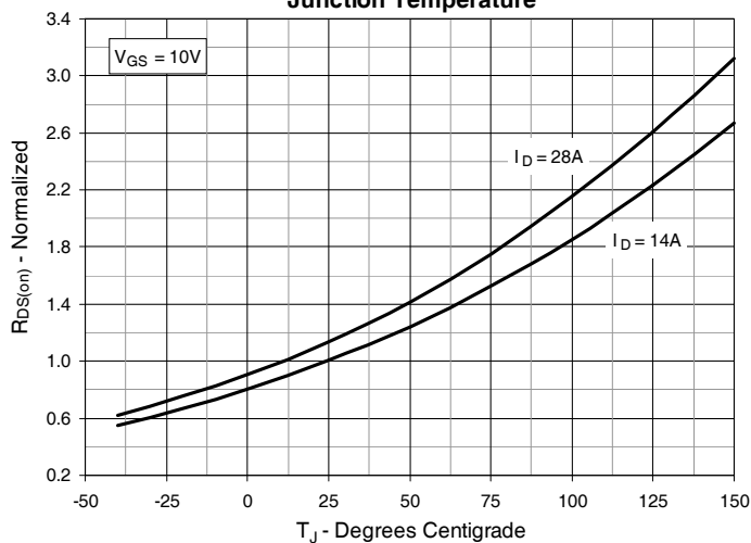
Fig. 4. R_{DS(on)} Normalized to I_D = 14\text{A} Value vs. Junction Temperature
