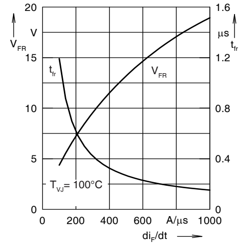
Fig. 23. Peak forward voltage V_{FR} and t_{fr}
