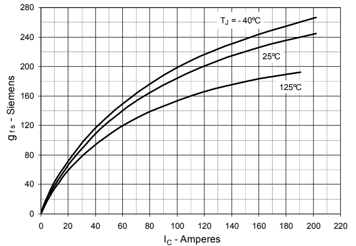
Fig. 6. Transconductance
