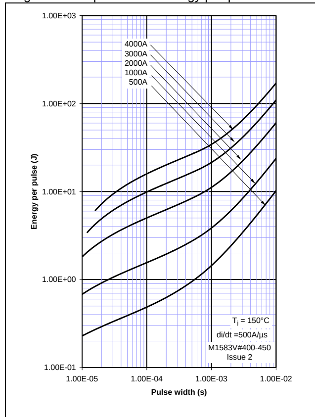
Figure 16 - Square wave energy per pulse
