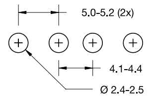
mounting pattern
