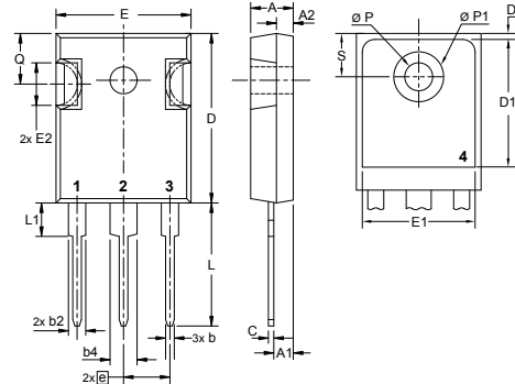
L014a TO-247AD
