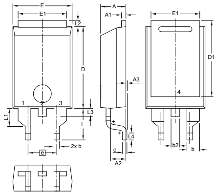
X013 PLUS220™ (SMD)
