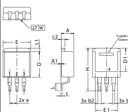
X011a TO-263 AA (D²PAK) Weight = 1.5 g
