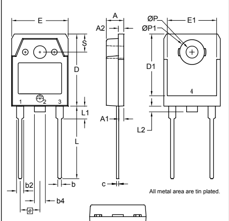
X017b TO-3P Weight = 5.5 g
