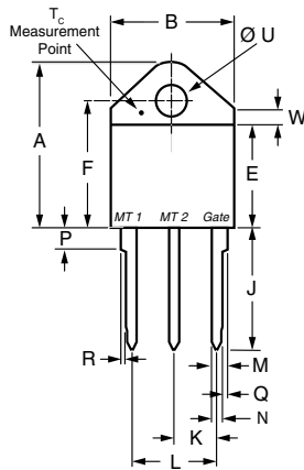
L002 TO-218AC Weight = 5 g
