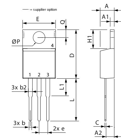
X005a TO-220 AB Weight = 2 g
