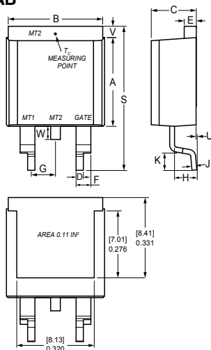
L011b TO-263AB Weight = 1.5 g
