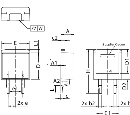
X011c TO-263 AB (D²PAK HV) Weight = 1.5 g
