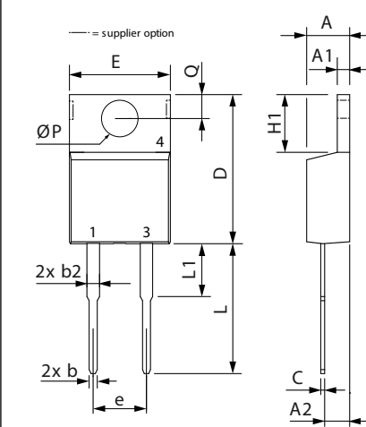
X005b TO-220 AC Weight = 2 g
