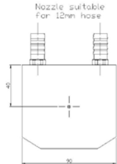
WCL15 - WS72-2 COOLER
