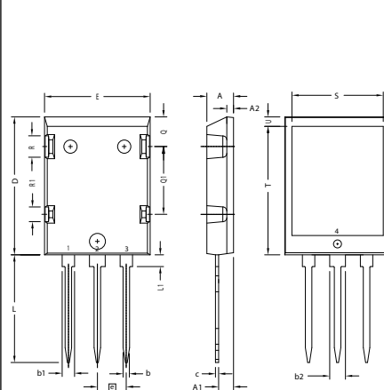
X022a ISOPLUS264™
