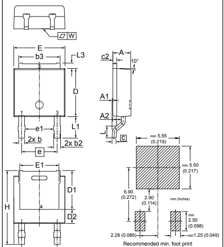
X004a TO-252 AA (D PAK HV) Weight = 0.3 g
