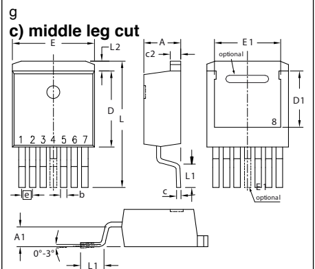
X012b TO-263 (7) Weight = 2.5 g
