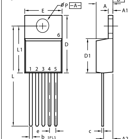
X006 TO-220 (5) Weight = 2 g
