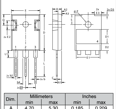
X016c ISO247™ Weight = 4.5 g
