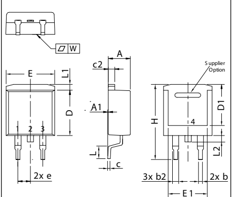
X011b TO-263 AB (D²PAK) Weight = 1.5 g
