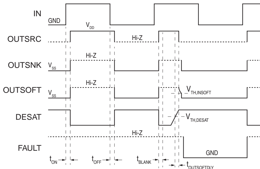
Figure 2. Timing Diagram
