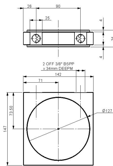
WCL11 - WS70 COOLER
