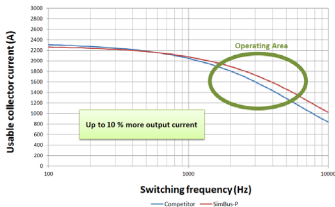
SimBus-P vs Competitor 1400A / 1200V
