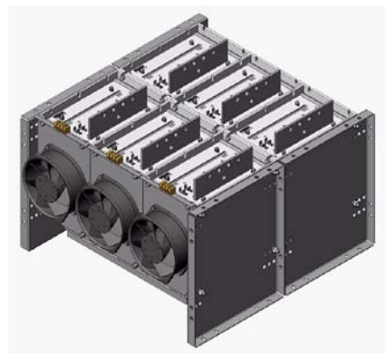
Figure 6 Weight 60 kg
