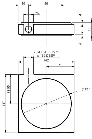
WCL10 - WS69 COOLER
