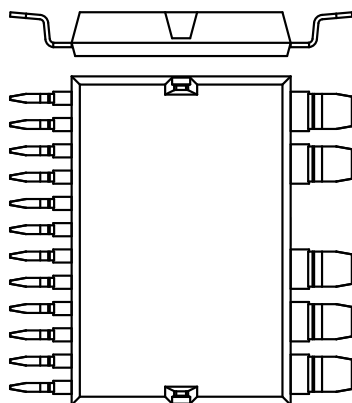
MTI...W...GC SURFACE MOUNT DEVICE
