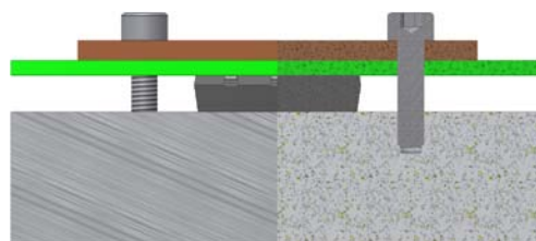
Fig. 4 Mounting example
