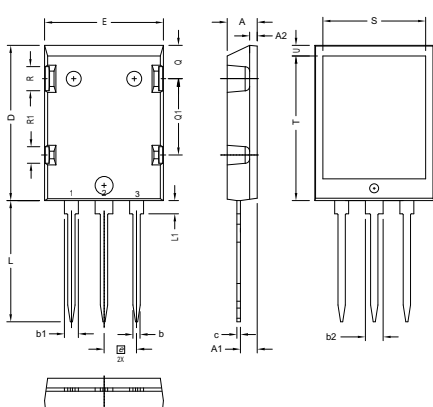
X022a ISOPLUS264™
