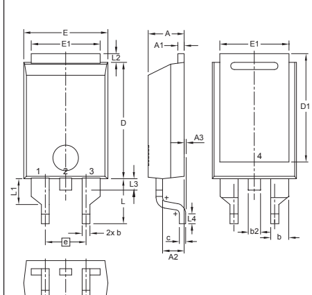
X013 PLUS220™ (SMD) Weight = 2 g
