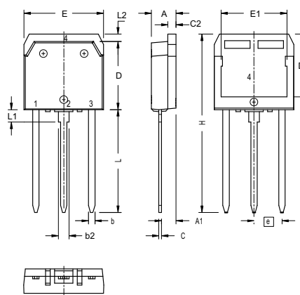
X018 TO-268 I 3 PAK Weight = 4.5 g
