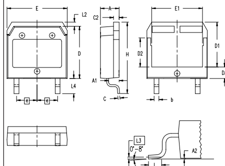
X019a TO-268 AA (D 3 PAK) Weight = 4 g
