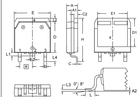
X019 TO-268 AA (D 3 PAK) Weight = 4 g
