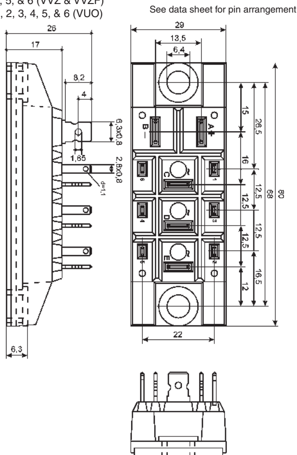
X121 PWS-C
