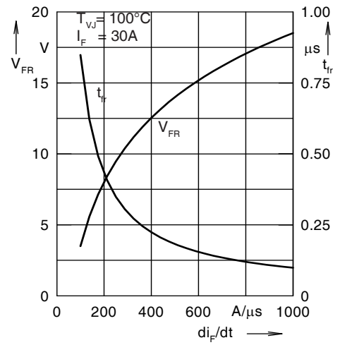
Fig. 19. Peak forward voltage V_{FR} and t_{fr} versus di_F/dt
