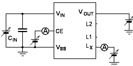
Circuit ⑤
