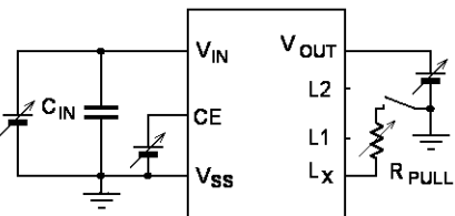
Circuit ⑦
