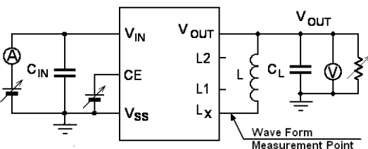
Circuit ⑧
