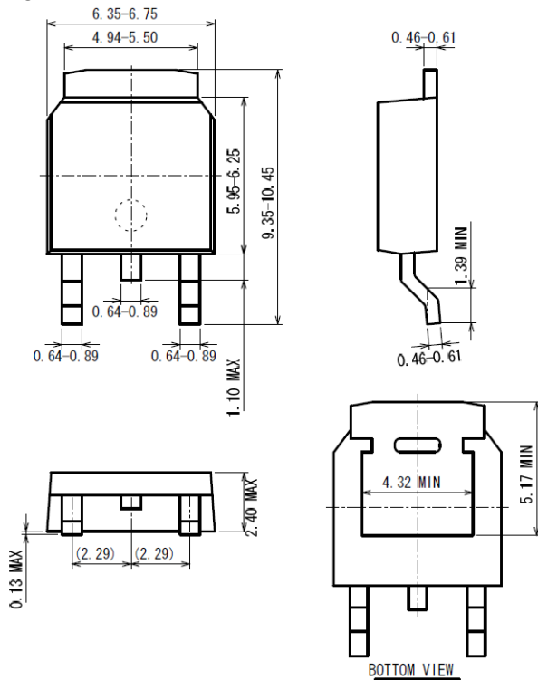
TO-252
