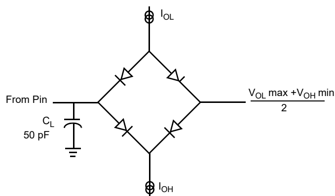
Figure 5. Test Load Diagram
