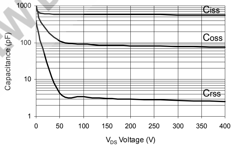
V_{DS} Voltage vs. Capacitance
