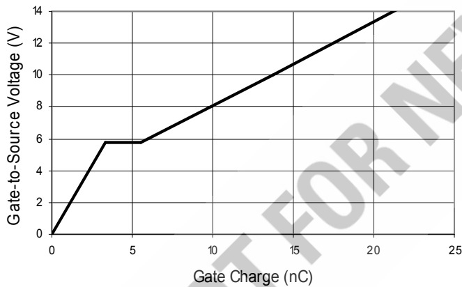
Gate Charge vs. Gate-to-Source Voltage V_{DS} = 250V , I_D = 2.25A
