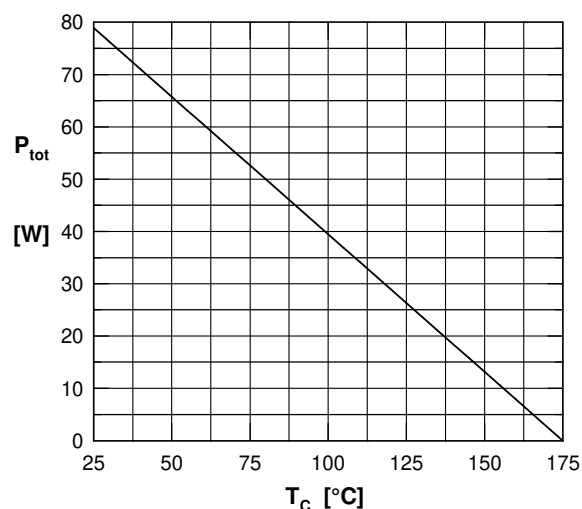
Fig. 4 Power derating
