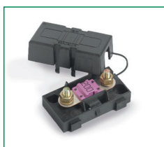
MIDI inline fuseholder (Left) MIDI covered fuseholder (Right)
