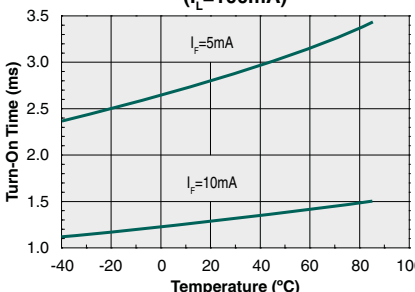
Typical Turn-On Time vs. Temperature ( I_L=100\text{mA} )
