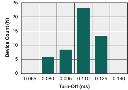
CPC1788 Typical Turn-Off Time (N=50, I_F=20\text{mA} , I_L=1\text{A}_{DC} , T_A=25^\circ\text{C} )
