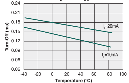
Typical Turn-Off vs. Temperature ( I_L=250\text{mA}_{DC} )
