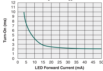
Typical Turn-On vs. LED Forward Current ( I_L=250\text{mA}_{DC} )
