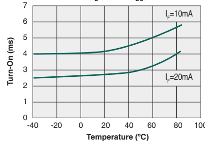
Typical Turn-On vs. Temperature ( I_L=250\text{mA}_{DC} )
