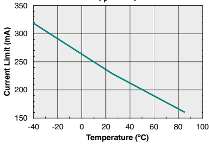
AC/DC Configuration Current Limit vs. Temperature ( I_F=5mA )
