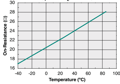
On-Resistance vs. Temperature ( I_F=5mA, I_L=100mA )
