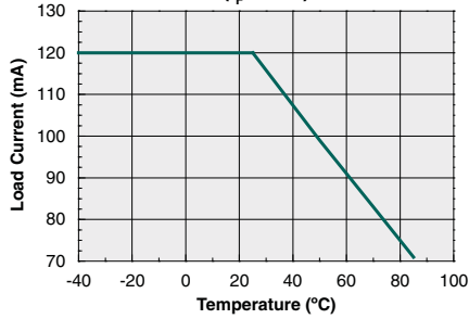
Typical Load Current vs. Temperature ( I_F=5mA )
