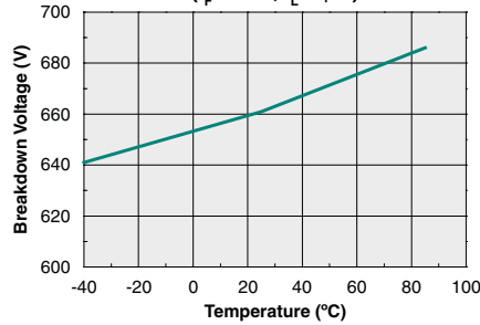
Switch Blocking Voltage vs. Temperature ( I_F=0mA, I_L=1\mu A )
