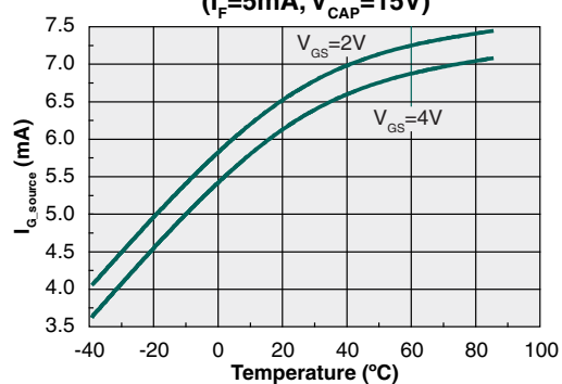
Gate Source Current vs. Temperature ( I_F=5\text{mA} , V_{CAP}=15\text{V} )
