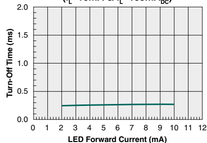
Typical Turn-Off Time vs. LED Forward Current ( I_L=10\text{mA} & I_L=100\text{mA}_{\text{DC}} )
