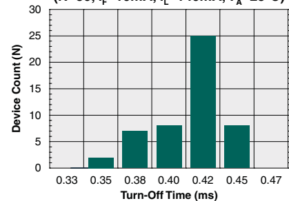
Typical Turn-Off Time (N=50, I_F=10\text{mA} , I_L=140\text{mA} , T_A=25^\circ\text{C} )
