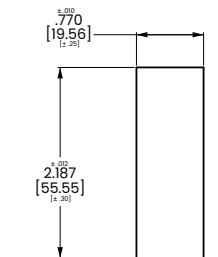
PANEL CUTOUT DETAIL
