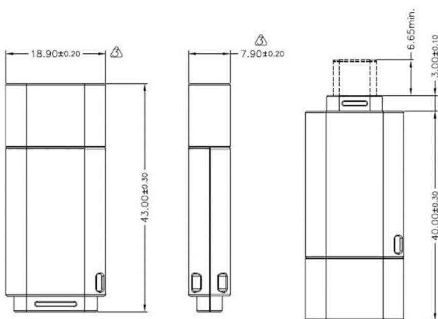
Figure 6-1 Physical Dimensions
