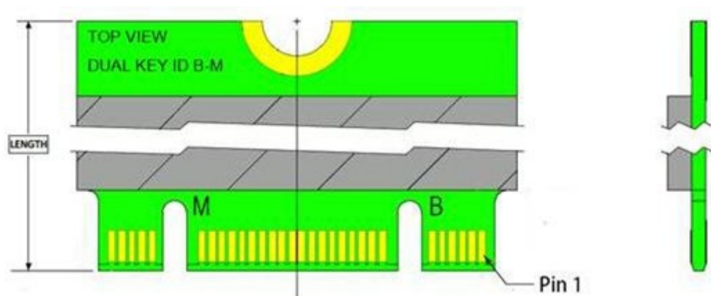
Figure 3-1 Pin Connectors
