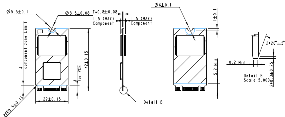
Figure 9-1 Dimensions
