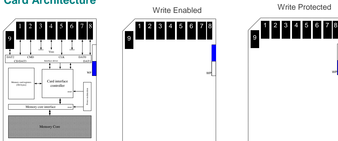
Figure 2-1 Card Architecture
