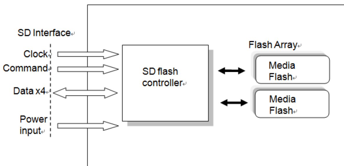
Figure 2-1 Block Diagram
