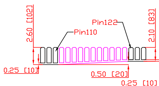
Detail D
